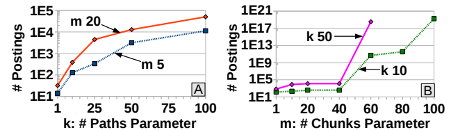
Figure 5: Number of postings (in logscale) from directly indexing one SFA. (A) Fix m , vary k . (B) Fix k , vary m . In (B), for k = 50 , the number of postings overflows the 64-bit representation beyond m = 60 .
